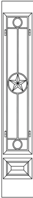
1'2" x 6'9" 3/4 Lite Sidelight
