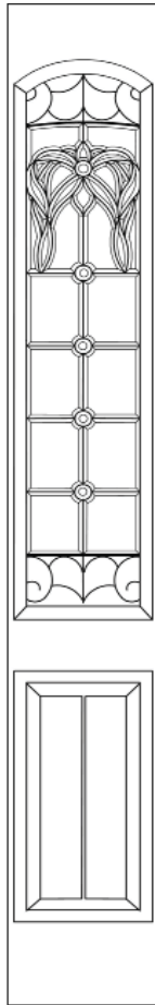
1'2" x 8'1" Arch 1/2 Lite Sidelight
