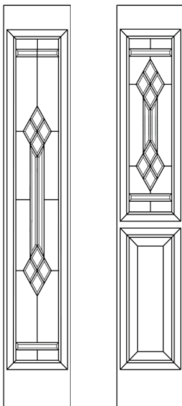
1'2" x 6'9" Full Lite Sidelight
