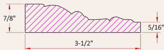
MCSG380 Mahogany Casing 8-0 104" KACSG380 Knotty Alder Casing 8-0 104"
