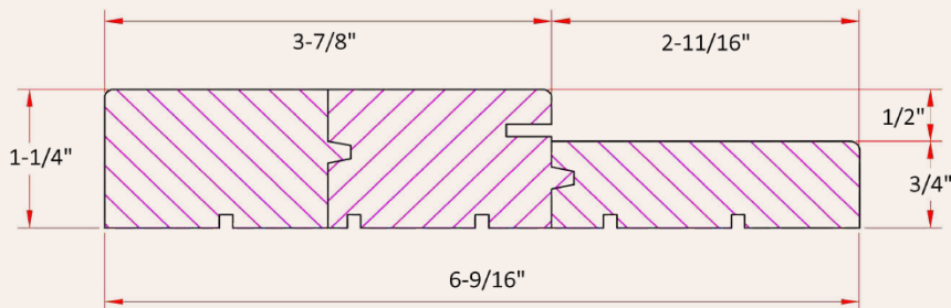
MJ680-2 6-9/16" Mahogany Jamb 8-0 100" (2-1/4" thick door) KAJ680-2 6-9/16" Knotty Alder Jamb 8-0 100" (2-1/4" thick door)
